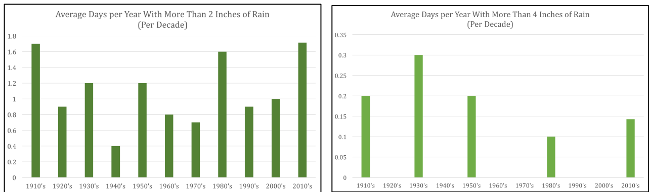
Figure 8: Average days in San Angelo, per decade, with more than two inches (left) and more than four inches (right) of rain. amount of rainfall events is displayed per decade.
