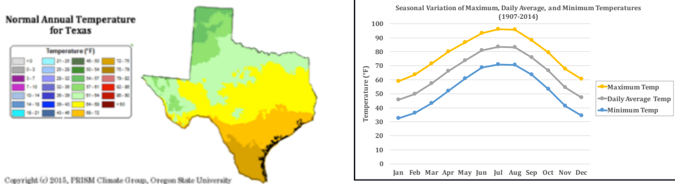
Figure 1: Texas average annual temperature in degrees F (left), and seasonal temperature variations for San Angelo showing maximum (yellow), daily average (gray), and minimum (blue) temperatures (right).
