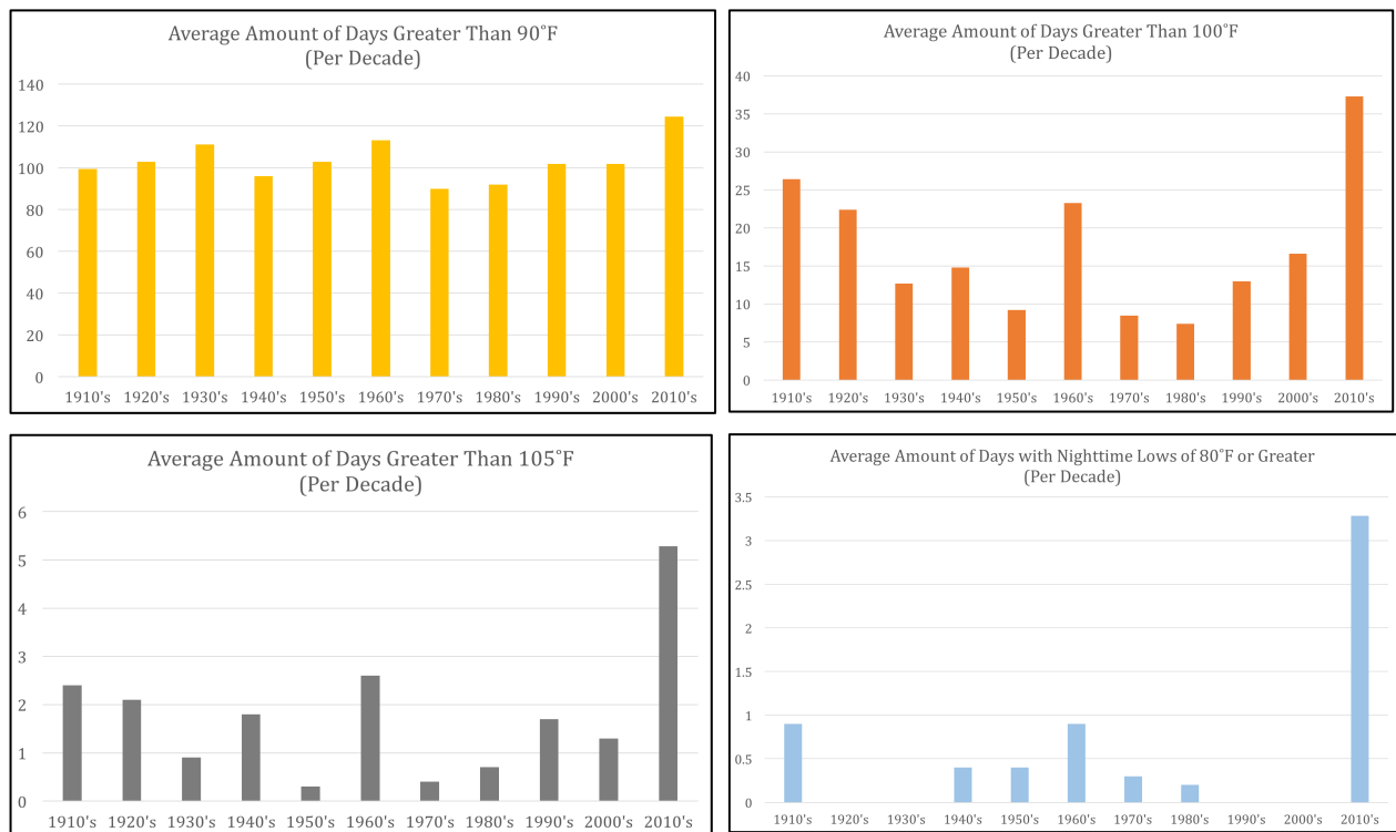
Figure 11: Average annual amount, per decade, of 90 degrees or greater (top left), 100 degrees or greater (top right) 105 degrees or greater (bottom left) and nighttime temperatures of 80 degrees or greater (bottom right).
