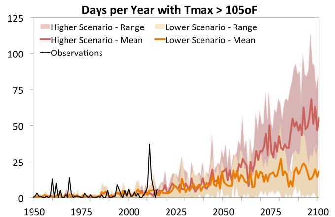
Figure 17: Projection of days with a maximum temperature at or above 105°F for a lower emissions scenario (orange line) and higher scenario (red line). Shaded areas indicate the range of model projections, and colored lines indicate the average of all models. Black line shows historical observations from 1950-2016.
