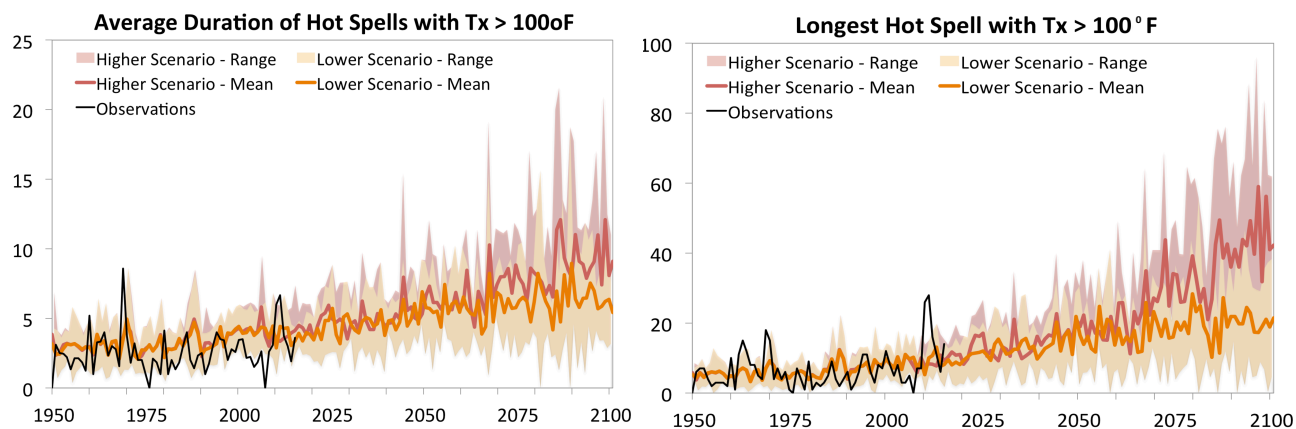
Figure 18: Projections of the average duration of heat waves and maximum length of heat waves, for days at or greater than 100°F, for a lower climate scenario (orange line) and a higher climate scenario (red line). Shaded areas indicate the range of model projections, and colored lines indicate the average of all models. Black line shows historical observations from 1950-2016.
