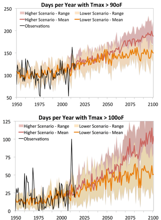
Figure 16: Projection of days with a maximum temperature at or above 90°F and 100°F for a lower emissions scenario (orange line) and higher scenario (red line). Shaded areas indicate the range of model projections, and colored lines indicate the average of all models. Black line shows historical observations from 1950-2016.
