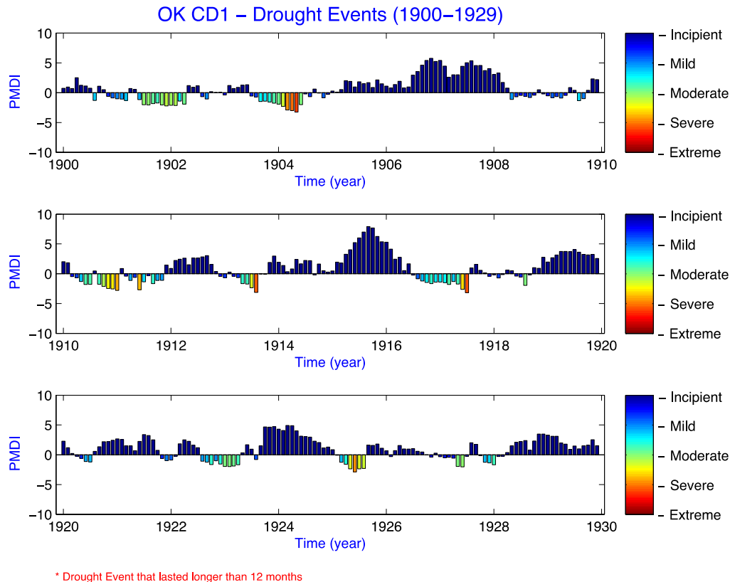
Fig. 1a. Drought event chronology and evolution from 1900-1929 for Climate Division 1.
