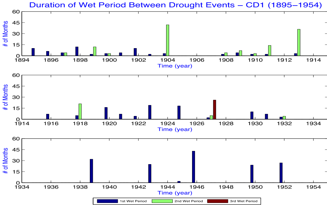
Fig. 2a. Breaks or wet periods each year, 1895-1954.
