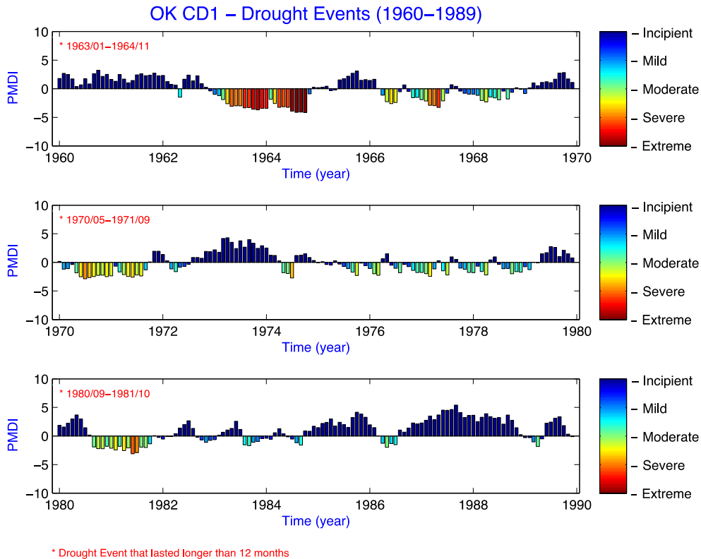
Fig. 1c. Same as Fig. 1a, but for 1960-1989 drought events.
