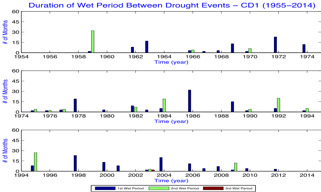
Fig. 2b. Same as Fig. 2a, but for 1955-2014.
