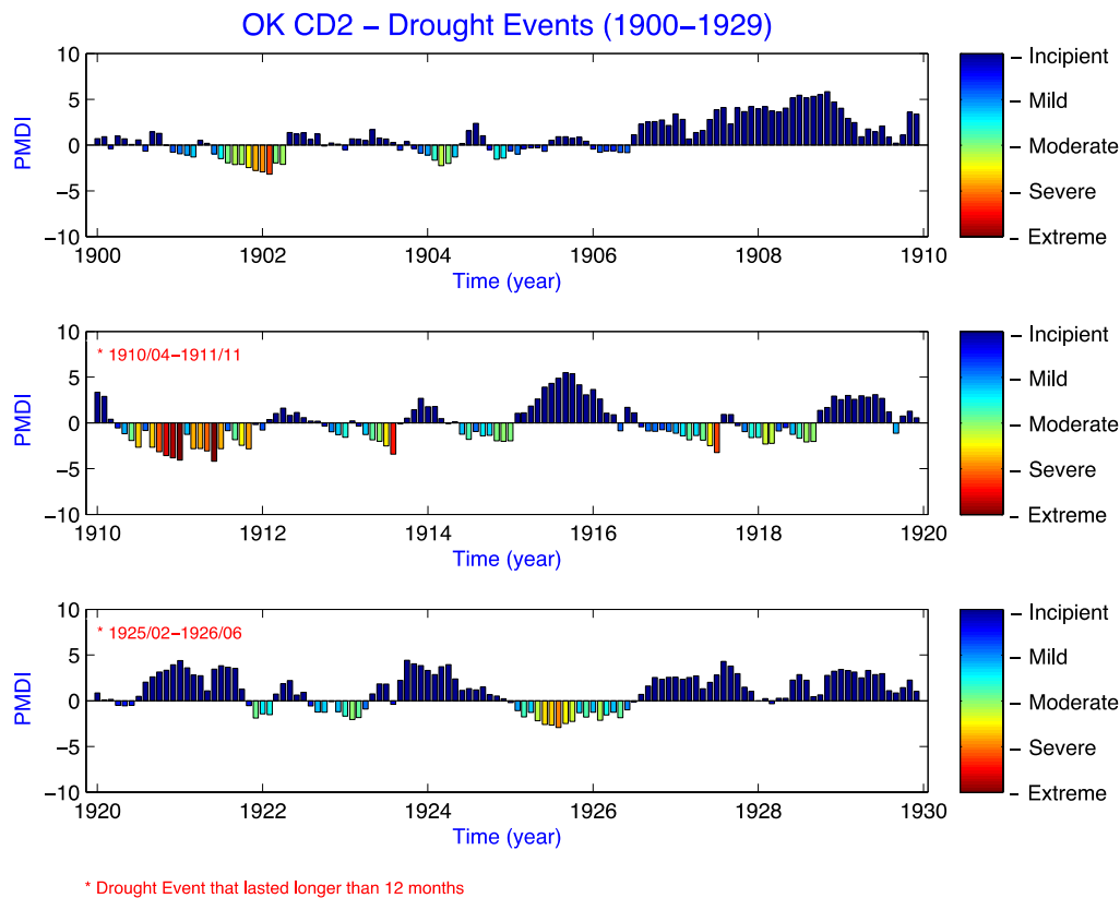
Fig. 1a. Drought events chronology and evolution from 1900-1929 for Climate Division 2.
