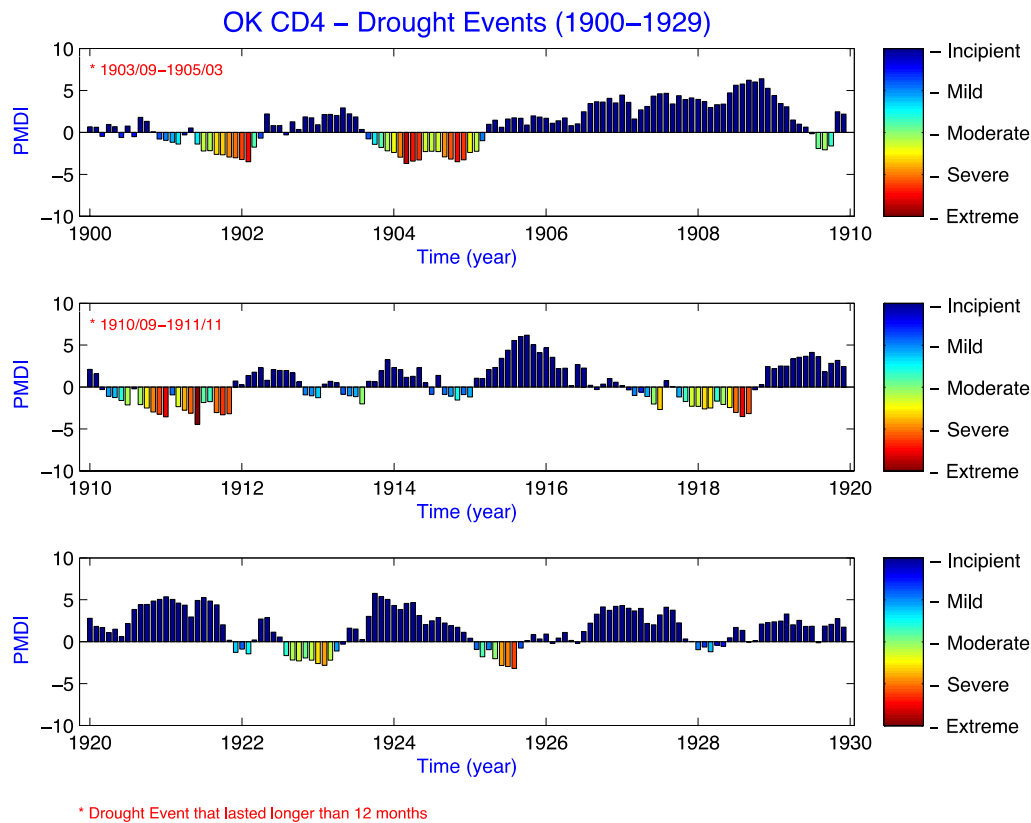
Fig. 1a. Drought events chronology and evolution from 1900-1929 for Climate Division 4.
