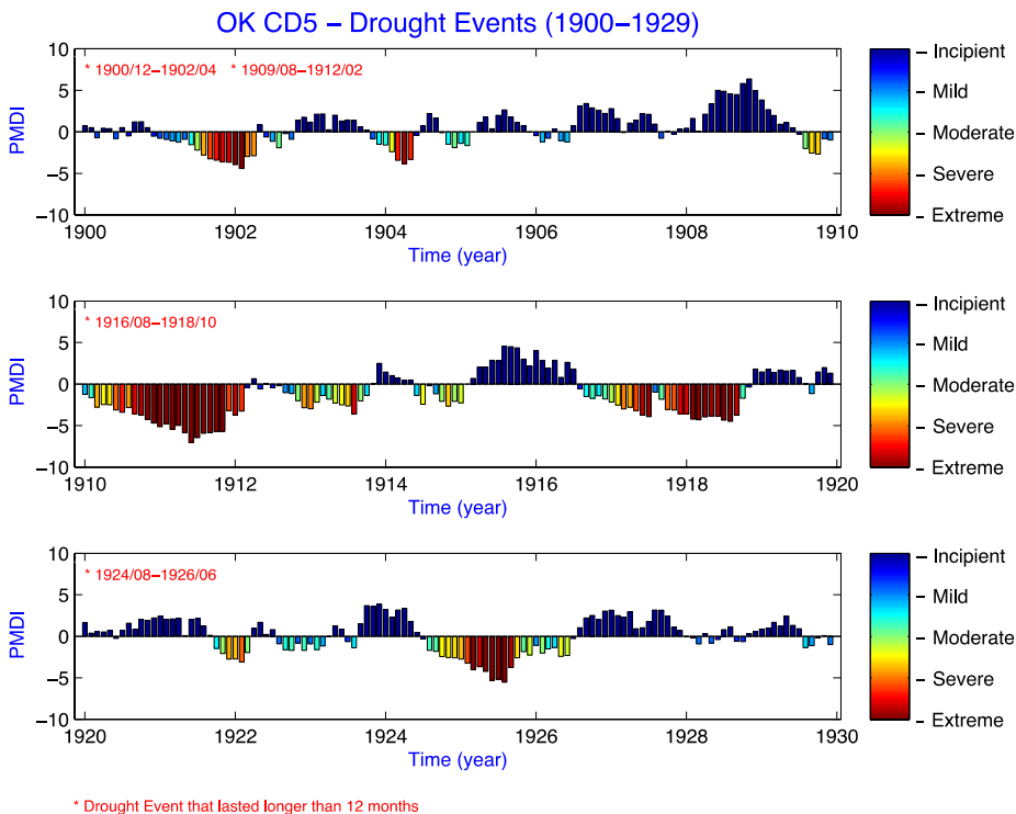
Fig. 1a. Drought events chronology and evolution from 1900-1929 for Climate Division 5.
