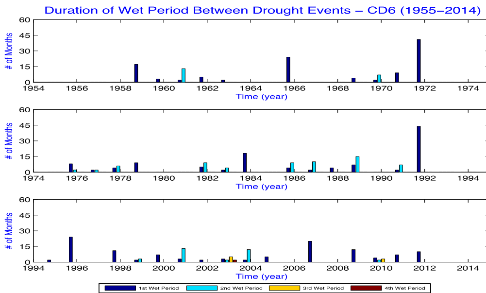
Fig. 2b. Same as Fig. 2a, but for 1955-2014.
