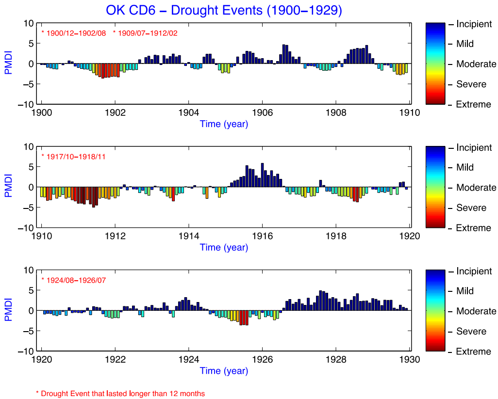
Fig. 1a. Drought events chronology and evolution from 1900-1929 for Climate Division 6.
