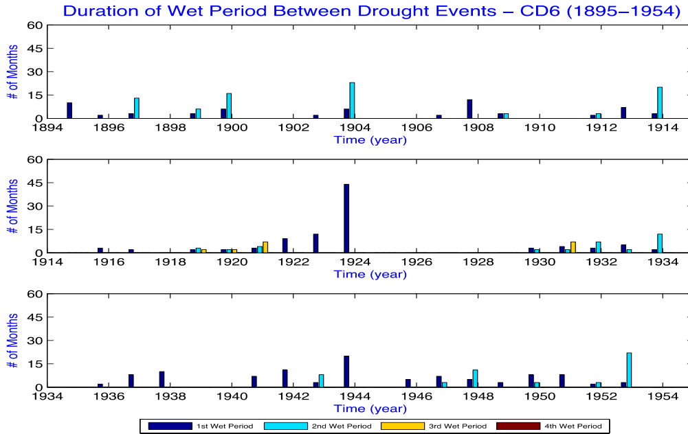
Fig. 2a. Breaks or wet periods per year.
