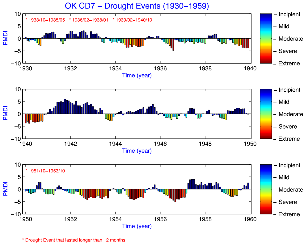
Fig. 1b. Same as Fig. 1a, but for 1930-1959 drought events.
