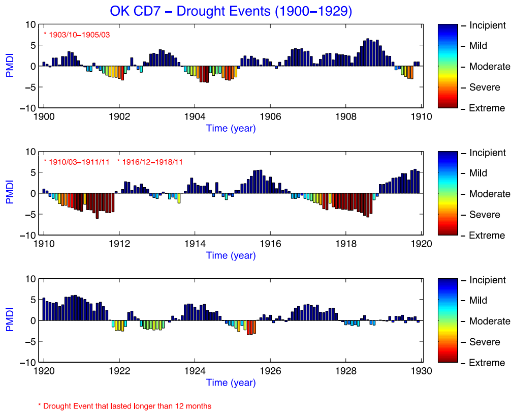
Fig. 1a. Drought events chronology and evolution from 1900-1929 for Climate Division 7.
