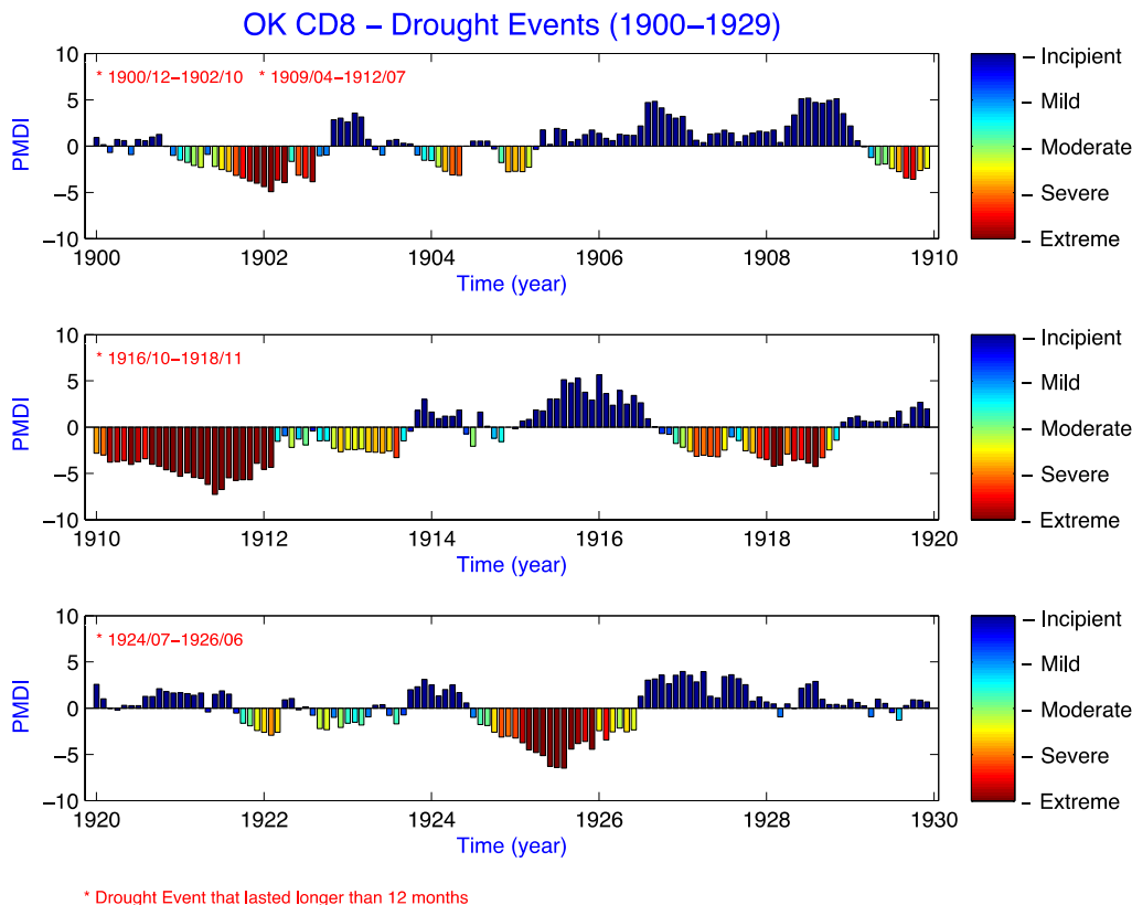
Fig. 1a. Drought event chronology and evolution from 1900-1929 for Climate Division 8.
