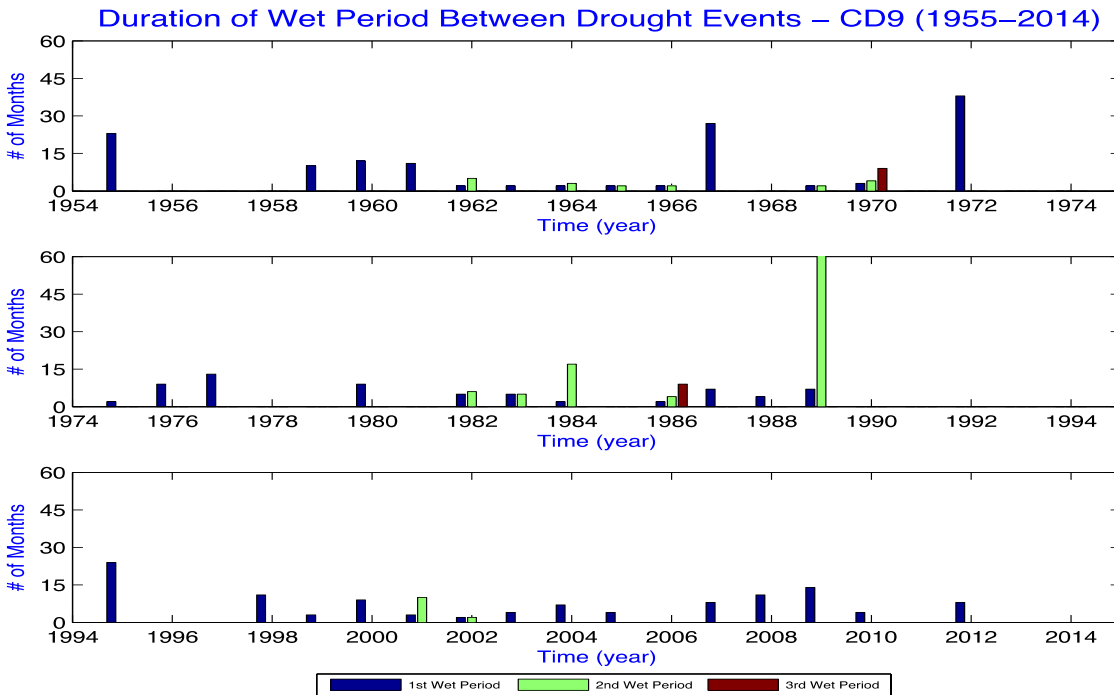
Fig. 2b. Same as Fig. 2a, but for 1955-2014.
