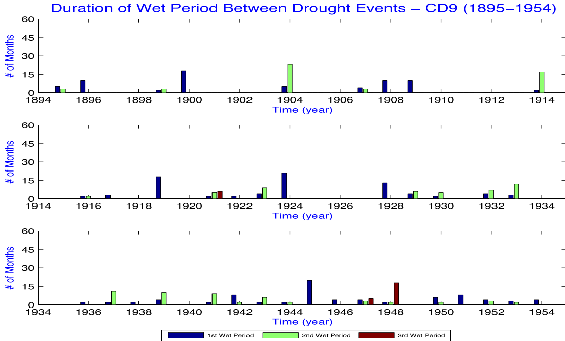
Fig. 2a. Breaks or wet periods per year.
