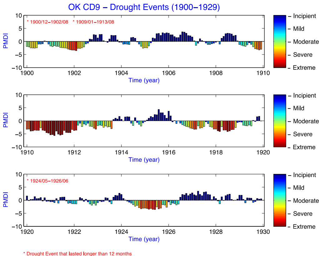
Fig. 1a. Drought events chronology and evolution from 1900-1929 for Climate Division 9.
